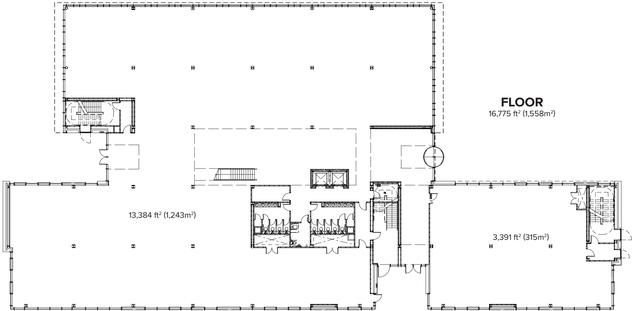
GROUND FLOOR PLAN NOT TO SCALE
